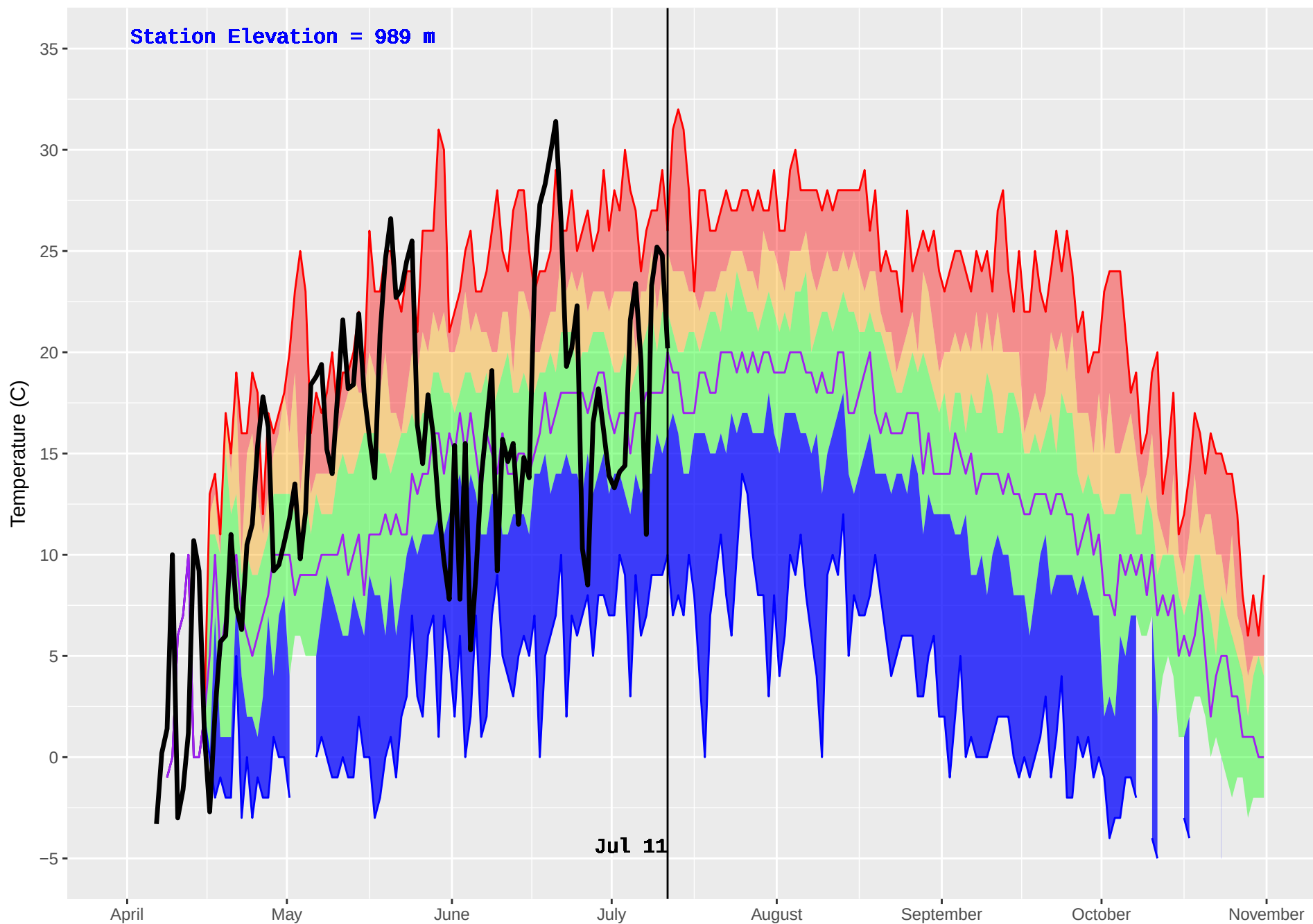
PINK MOUNTAIN (129) : Historical (1983–2016) and Current (2018) Noon Temperature
